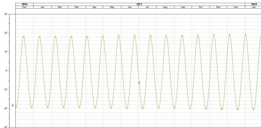
Figure 18 Moon Declination 2017
