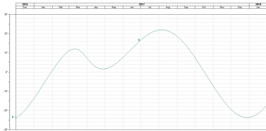
Figure 12 – Venus Declination 2017
