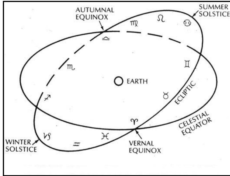
Figure 1 The Ecliptic
