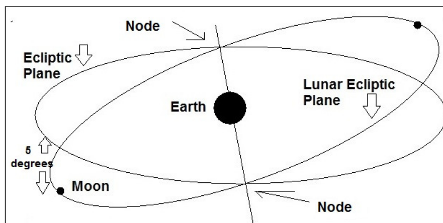
Figure 5 – The Nodes
