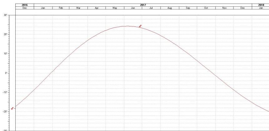
Figure 14 – Mars Declination 2017
