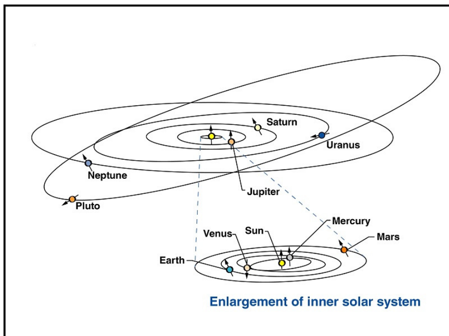
Figure 3 – The Planets
