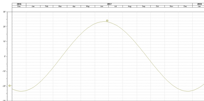
Figure 16 Sun Declination
