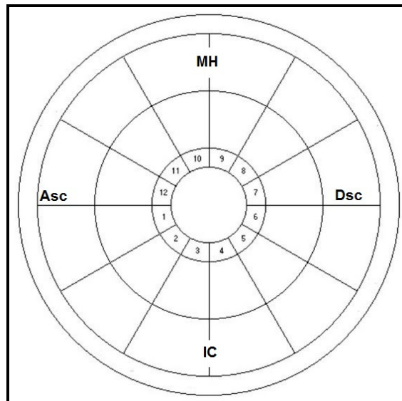
Figure 6 – Cardinal Points
